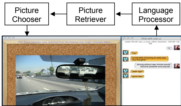
Figure 2. IdeaExpander screenshot and high-level architecture. The system monitors the group conversation (right) and selects pictures to display to the group (left).
